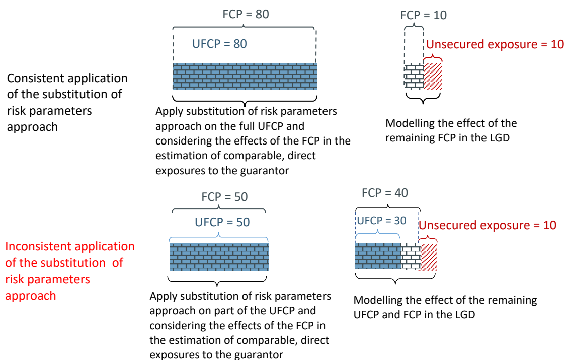
Figure 5: Application of the substitution of risk parameters approach based on allocation A described in Figure 4
