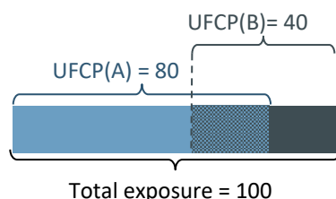
Figure 8: Application of the substitution of risk parameters approach based on the allocation described in Figure 7
